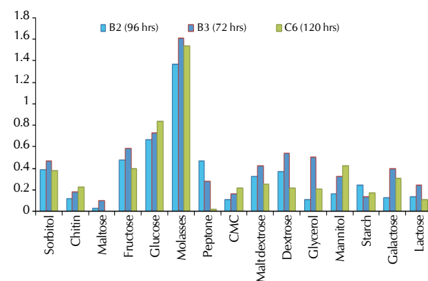
Figure 2: Effect of different carbon sources on PHB (expressed as Crotonic acid (O.D. 235))
