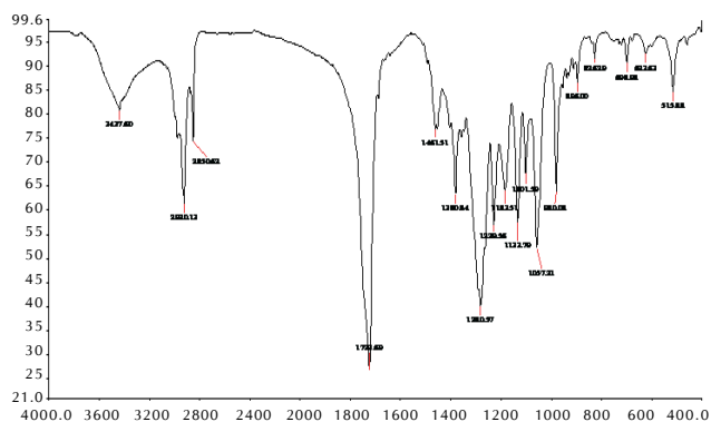
Figure 4: FTIR spectrum of PHB produced by strain B3 peaks at 29
