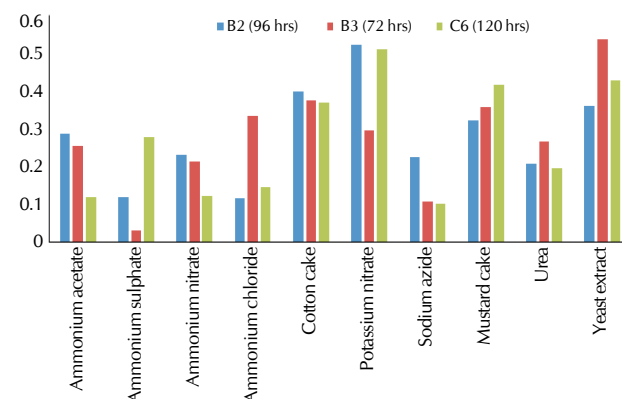
Figure 3: Effect of different nitrogen sources on PHB (PHB expressed as Crotonic acid (O.D. 235))
