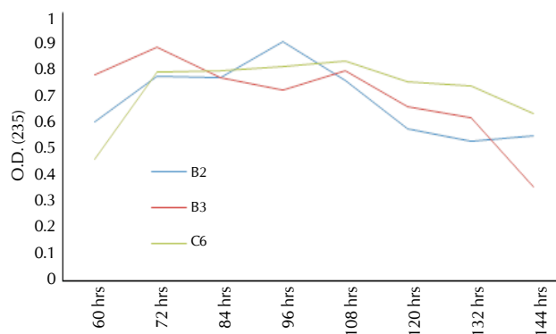
Figure 1: Kinetics of PHB production in three strains expressed as Crotonic acid (O.D. 235)
